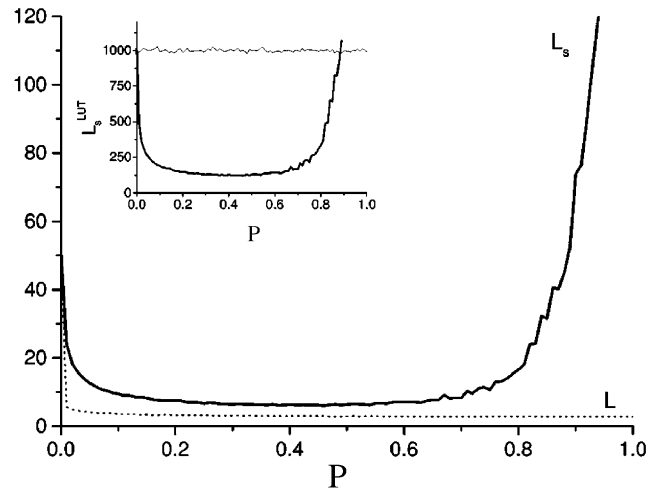
Fig. 7.9. Search time L_s (solid line), and average shortest path length L (dashed line), as a function of the rewiring probability p for a WS small-world network with N = 2000 nodes and K = 10\,000 links. The inset shows L_s^{\text{LUT}} for the search method adopted in Ref. [865] (thick line) and for the breadth-first search method (thin line). Reprinted figure with permission from Ref. [865]. © 2003 by the American Physical Society.
