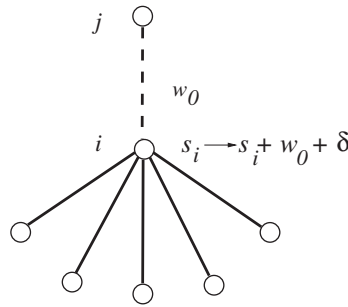
Fig. 2.7. Reprinted figure with permission from Ref. [214] BBV model. © 2004 by the American Physical Society. Local rearrangement of weights due to the presence of the new node j and the new link l_{ji} . The weight of the new edge is w_0 and the total weight on the existing edges connected to i is modified by an amount equal to \delta .
