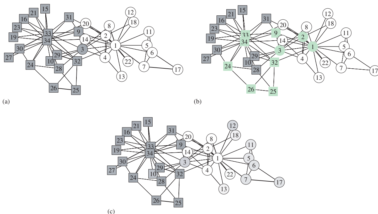
Fig. 7.1. Finding community structures in the karate club network of Zachary. The numbered vertices of the network represent the members of the club, while the edges represent friendships, as determined by the observation of the interactions [837]. The two groups into which the club split during the course of the study are indicated by the squares and circles, while the dark grey and white show the divisions of the network found by (a) the spectral bisection algorithm of Section 7.1.1, (b) the hierarchical clustering method of Section 7.1.2 and (c) the Monte Carlo sampled version of the algorithm of Girvan and Newman proposed by Tyler et al. and discussed in Section 7.1.4. In (b) the lightly shaded vertices are those not assigned by the algorithm to either of the two principal communities. In (c) shades intermediate between the dark grey and white indicate ambiguously assigned vertices that fall in one community or the other, or neither, on different runs of the algorithm. Reprinted figure with permission from [829]. © 2004 by the European Physical Society.
