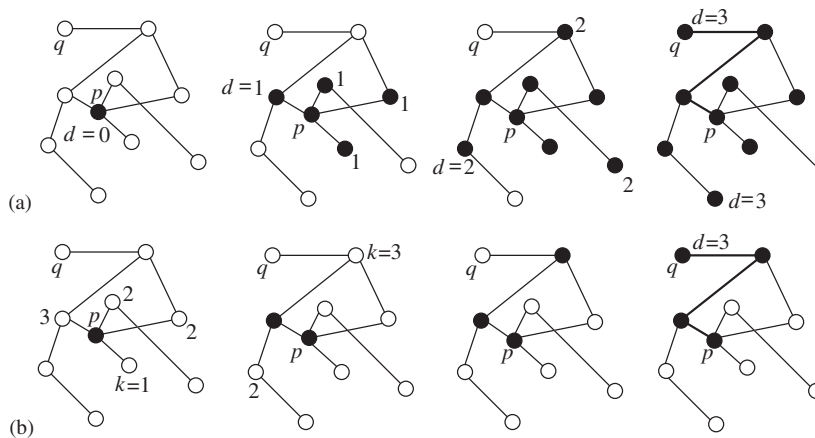
Fig. 7.7. Schematic diagram of (a) the breadth-first search algorithm and (b) the maximum degree strategy for searching from node p to node q . In all cases d denotes the step number of the algorithm. Reprinted figure with permission from Ref. [861]. © 2002 by the American Physical Society.
